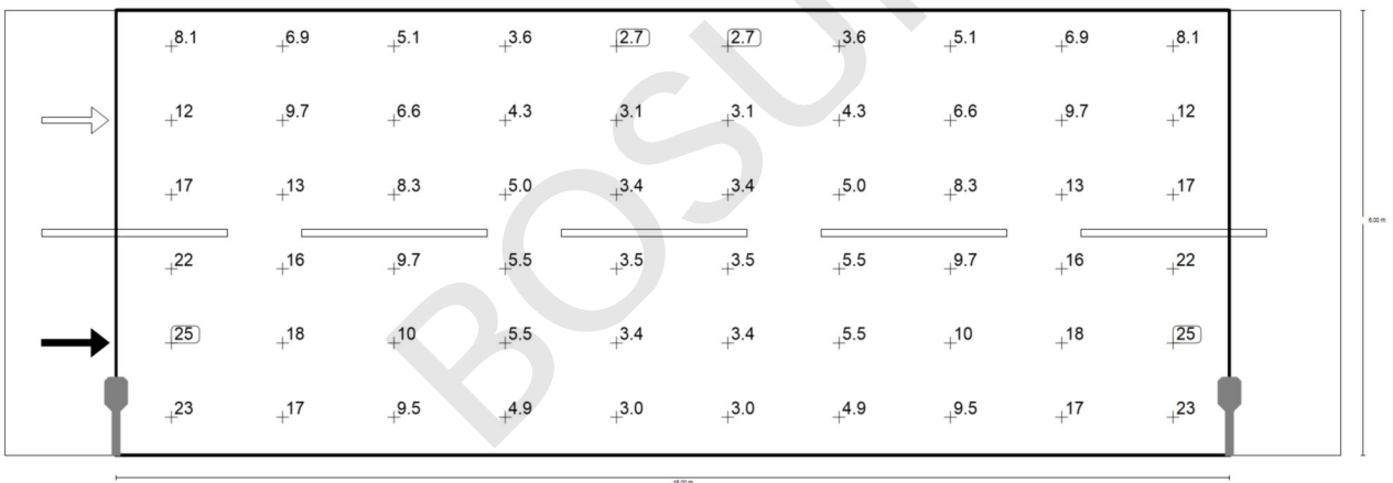
Maintenance value, horizontal illuminance [lx] (Value grid)
