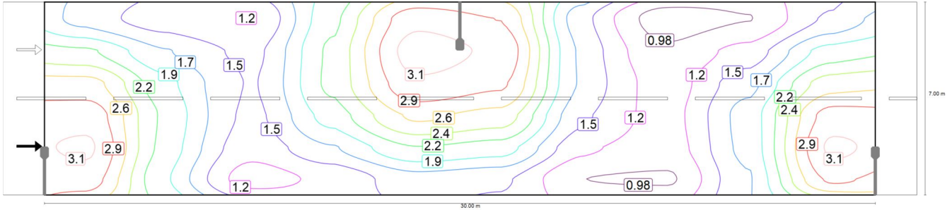
Observer 1: Maintenance value, luminance with dry roadway [cd/m 2 ] (Iso-illuminance curves)
